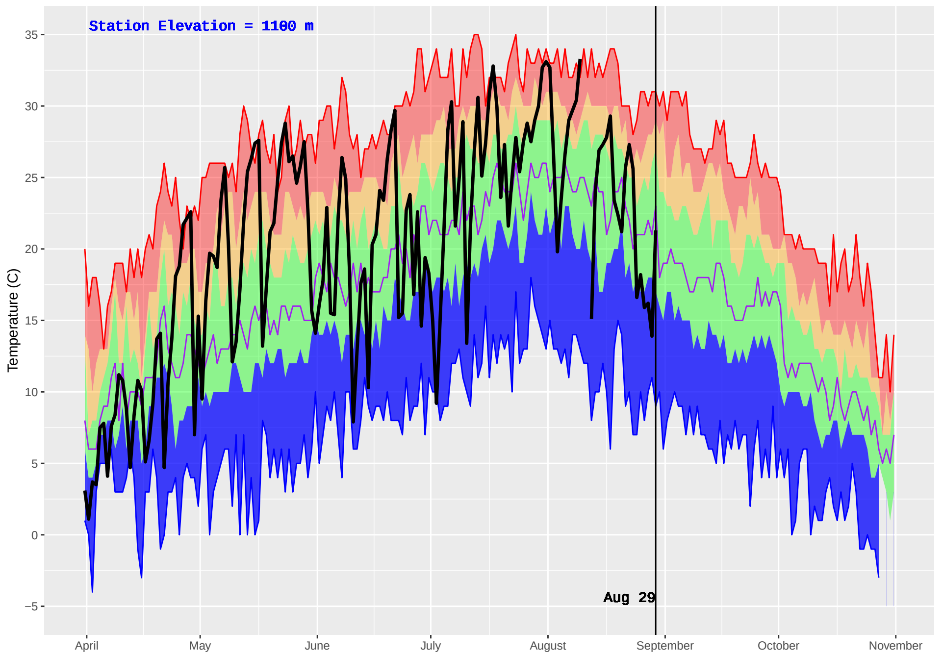
PALLISER (411) : Historical (1973–2016) and Current (2018) Daily Temperature
